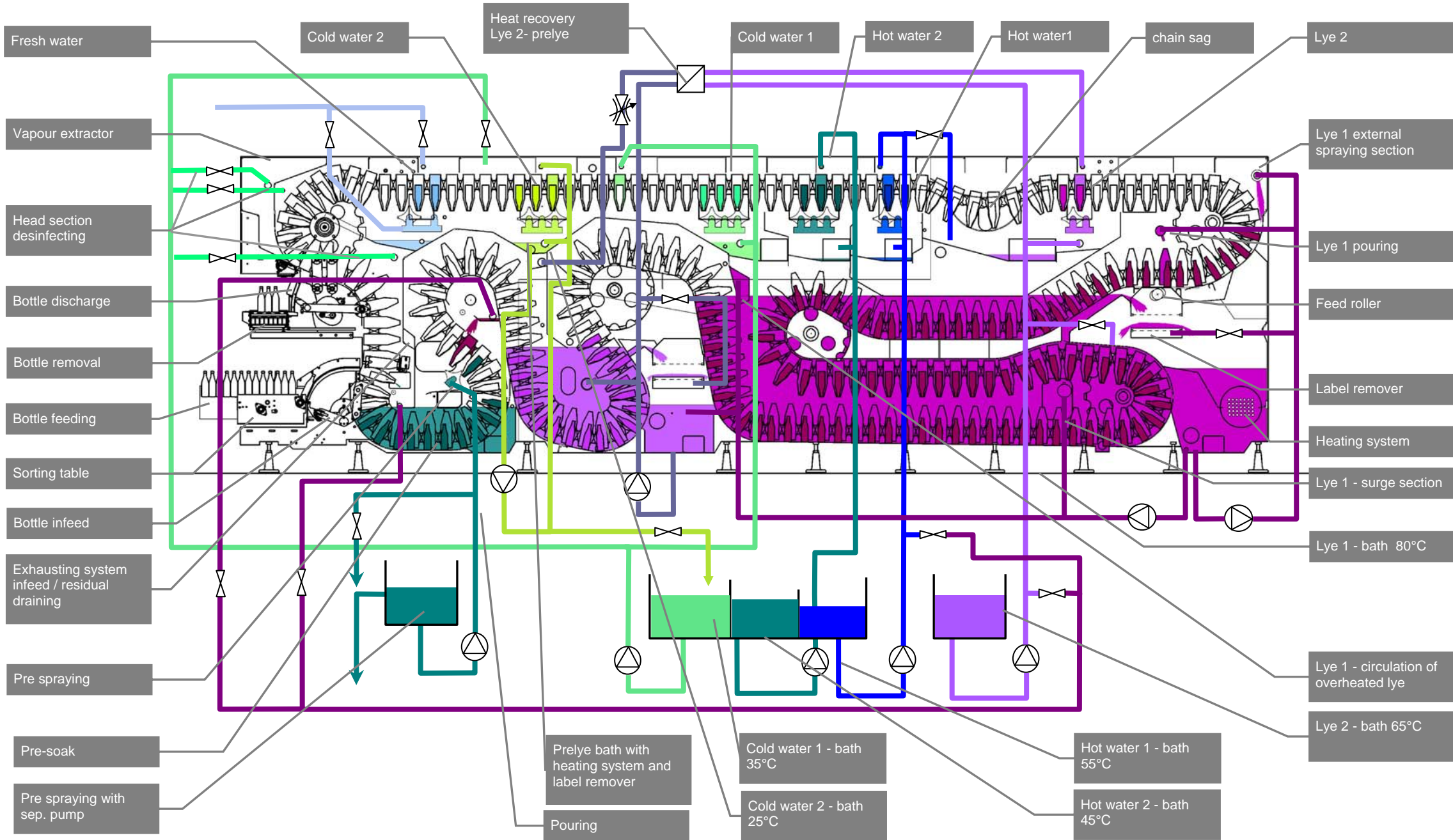
Heating by external plate heat exchanger (optional)
